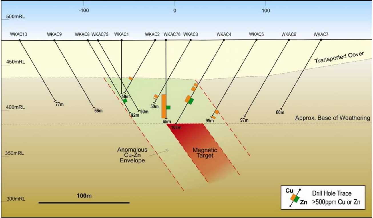
Figure 2 Defiance Cross Section
