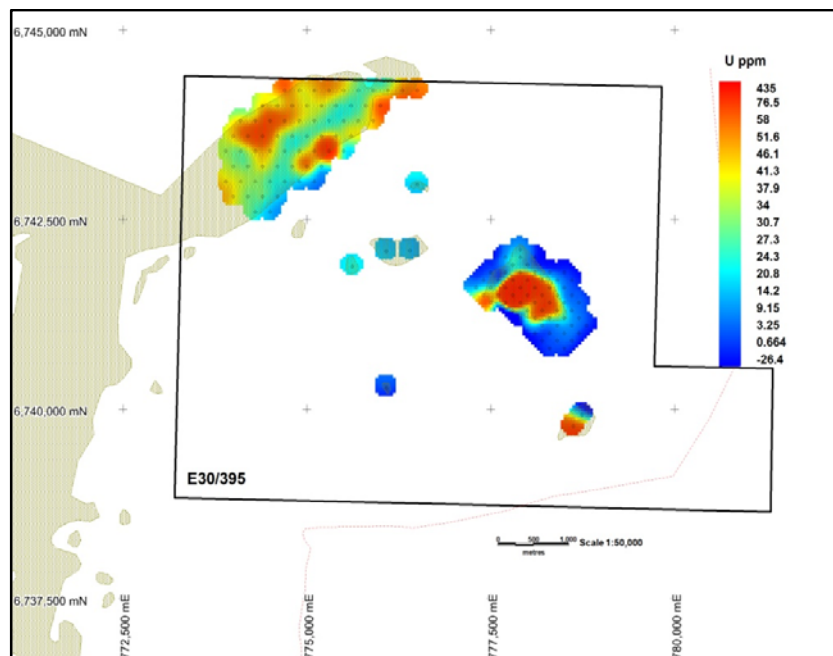
Barlee South Uranium in Soil Geochemistry
